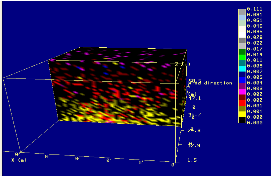
Fig. 6. Computed spatial patterns of solids concentration in the vertical plane at 500 m downwind from the source under conditions specified in report.
